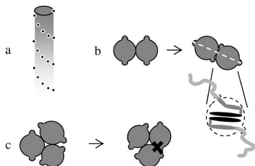
FIGURE 6 ( a ) Cartoon depicting a protofilament with protrusions, representing the locations of the disordered residues 1–17. ( b ) Cross sections through a fibril consisting of two protofilaments that demonstrates a possible mechanism by which steric overlap between protofilaments is avoided. ( c ) Cross sections through a threefold fibril. Here, the mechanism described for twofold fibrils does not apply.
