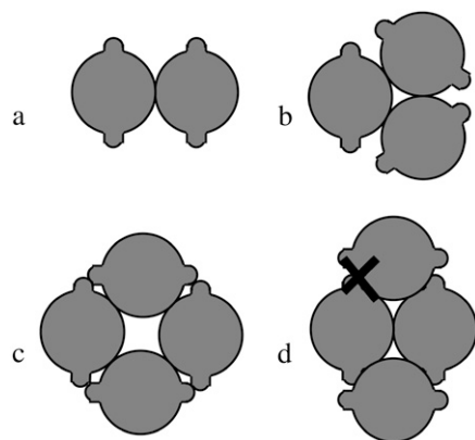
FIGURE 5 Interactions of cylinders with protrusions, linked to the places where the disordered chain emerges from the protofilament. Panels a , b , and c show geometries in which there is no steric overlap. Geometry d , however, is forbidden in our model due to steric overlap.
