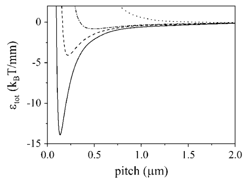
FIGURE 1 Energy of intertwining versus pitch, for a bundle of two rods. We use a value of -10 k_B T/\text{nm} for \epsilon_{\text{int}} , and vary the Young's bending modulus. The drawn line corresponds to Y = 0.5 GPa, the dashed line to Y = 1 GPa, the dot-dash line to Y = 5 GPa, and the dotted line to Y = 100 GPa.
