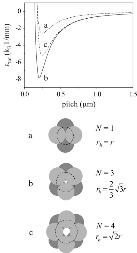
FIGURE 2 Energy of intertwining versus pitch, for bundles of rods of the three geometries depicted. We use a value of 1 GPa for the Young's modulus and a value of -8 \text{ k}_B\text{T/nm} for \epsilon_{\text{int}} . Lines correspond to the geometries pictured, as indicated.
