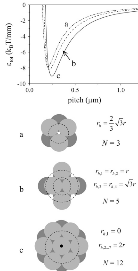
FIGURE 3 Energy of intertwining versus pitch, calculated with Eq. 5, for the three geometries depicted. We use a value of 1 GPa for the Young's modulus and a value of -8 \text{ k}_B\text{T/nm} for \epsilon_{\text{int}} . Lines correspond to the geometries pictured, as indicated.
